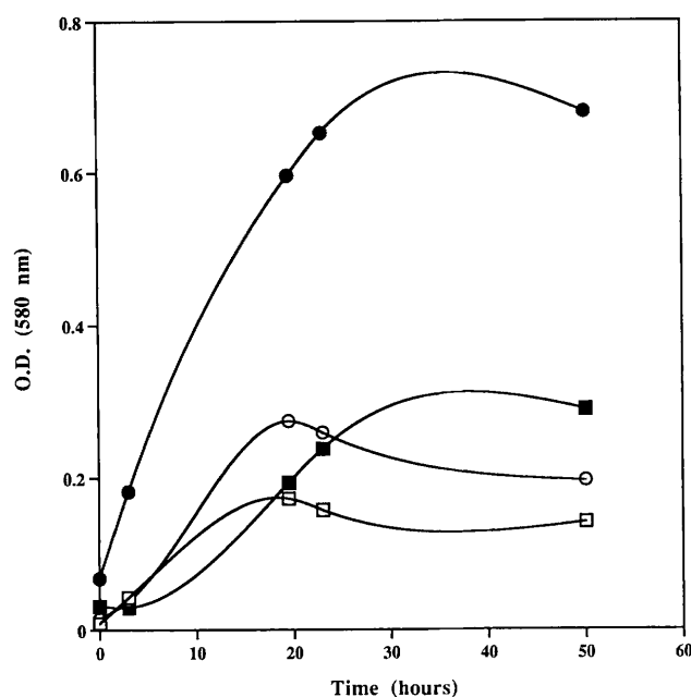
FIG. 1. Effect of thiosulfate on the growth of Thermosipho africanus cultivated in basal medium containing 1 g of yeast extract per liter and 1 g of bio-Trypticase per liter. Symbols: \square , control; \circ , 20 mM thiosulfate; \blacksquare , 20 mM glucose; \bullet , 20 mM glucose plus 20 mM thiosulfate. O.D. (580 nm), optical density at 580 nm.
