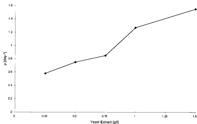
FIG. 3. Effect of yeast extract concentration on the specific growth rate ( \mu ) of strain Z-7935 T .
