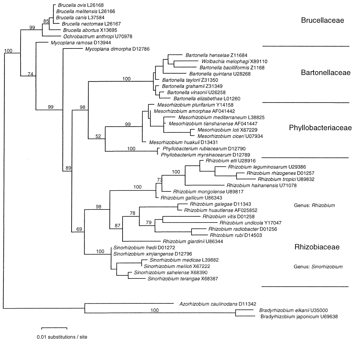
Fig. 1. Maximum-likelihood tree expressing the relationships among the Rhizobiaceae and their relatives, based on 16S rDNA sequences. Horizontal branch lengths are proportional to the estimated number of nucleotide substitutions and local bootstrap probabilities (as percentages) were determined for 1000 resamplings. Bacterial family names are those recorded on the website of the Bergey's Manual Trust ( http://www.cme.msu.edu/Bergeys ).
