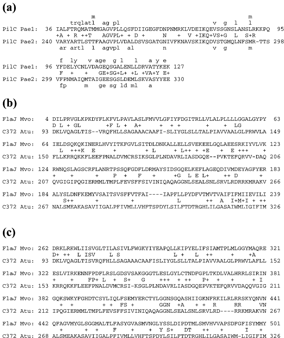
Fig. 7. Binary sequence alignments revealing the sequence similarities between (a) the two repeat sequences within a representative bacterial multispansing TM protein, the PilC protein of P. aeruginosa , (b) the first half of the archaeal FlaJ protein of M. voltae and second half of the bacterial C372 protein of A. tumefaciens and (c) the second half of the archaeal FlaJ protein of M. voltae and the bacterial C372 protein of A. tumefaciens . Residue number in each protein is provided at the beginning and end of each line. Residues identical in the two sequences are shown between the binary alignments while conservative substitutions are displayed with a '+'. In Fig. 7(a), residues indicated in lower-case characters above and below the alignment are amino acids that are highly conserved in the first and second halves, respectively, of most members of the T2SF-PilC/G-PilR clusters of proteins.
