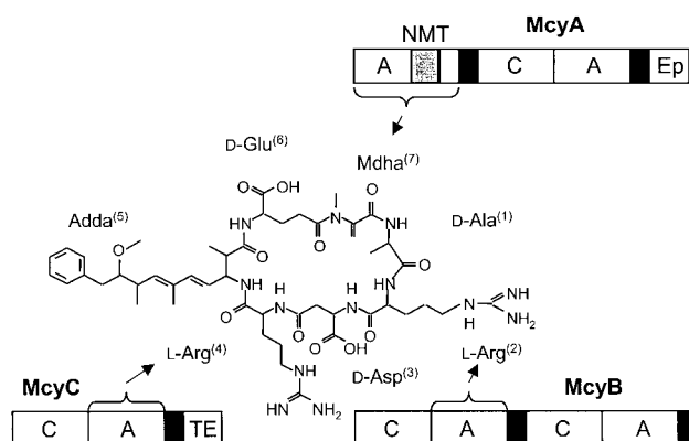
Fig. 1. Structure of [Asp 3 , Mdha 7 ]-MC-RR and the multi-enzymes McvA, McvB and McvC believed to be responsible for the collinear activation and incorporation of Mdha 7 , D-Ala 1 , L-X 2 , D-MeAsp 3 and L-Z 4 during biosynthesis (Tillett et al. , 2000). Each rectangle represents a non-ribosomal peptide synthetase enzymic domain: A, aminoacyl adenylation; C, condensation; NMT, N-methyl transferase; Ep, epimerase; TE, thioesterase. Thiolation domains are shown in black. Braces indicate the adenylation domains sequenced from Planktothrix strains (see Table 1) and arrows denote the corresponding amino acids activated during biosynthesis.
