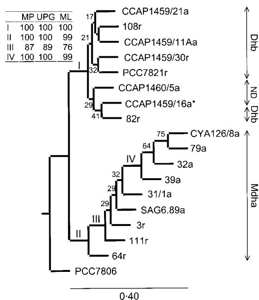
Fig. 2. Phylogenetic tree based on MP analysis calculated from mcvAAd1 sequences (950 aa) from 17 Planktothrix strains. Significant bootstrap percentages obtained from 1000 replicates are indicated for mcvA clades I, II, III and IV at the top left for MP, UPGMA clustering (UPG) and ML. Bootstrap values for clades with lower support are given for MP only. mcvAAd1 from Microcystis PCC7806 (AAF00960) was used as an outgroup. The suffixes r and a after the strain name indicate the species P. rubescens (r) and P. agardhii (a). The corresponding amino acids in position 7 determined in the MC molecule are given (ND, not determined). Bar, 4 substitutions per 10 amino acids. [Asp 3 , Dhb 7 ]-MC-HtyR has been isolated from strain CCAP1459/16 (indicated by an asterisk) by Sano & Kaya (1998).
