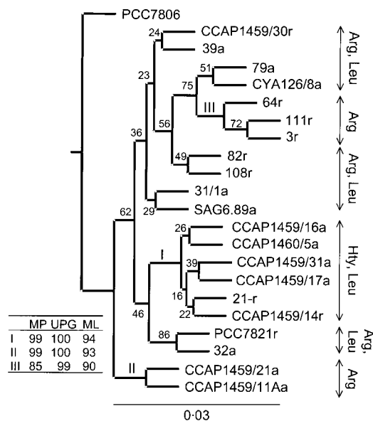
Fig. 3. Phylogenetic tree based on MP analysis calculated from mcvBAd1 sequences (513 aa) from 21 Planktothrix strains. Bootstrap percentages obtained from 1000 replicates are indicated for mcvB clades I, II, III at the bottom left for MP, UPGMA clustering (UPG) and ML. Bootstrap values for clades with lower support are given for MP only. mcvBAd1 from Microcystis PCC7806 (AAF00961) was used as an outgroup. The suffixes r and a after the strain name indicate the species P. rubescens (r) and P. agardhii (a). The corresponding amino acids in position 2 determined in the MC molecule are given. Bar, 0.3 substitutions per 10 amino acids.
